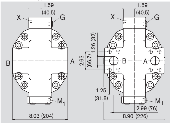
Service line ports A/B at side, opposite (52)
