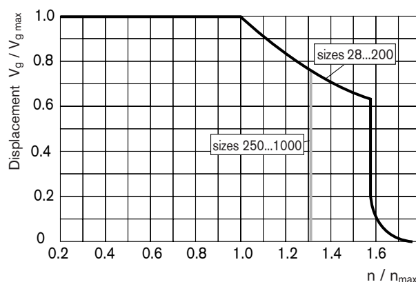
Permitted displacement in relation to rotational speed
