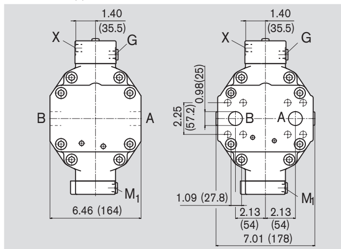
View Z
