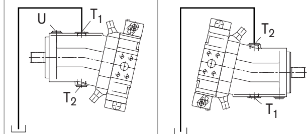
Installation position 1
