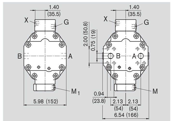
View Z
