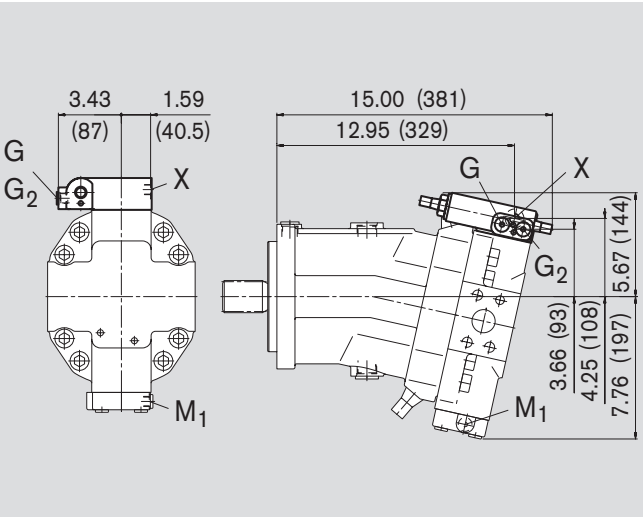
Electrical control with proportional solenoid EP1, EP2
