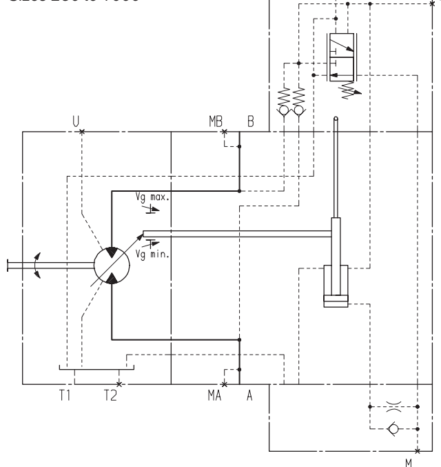
Sizes 250 to 1000
