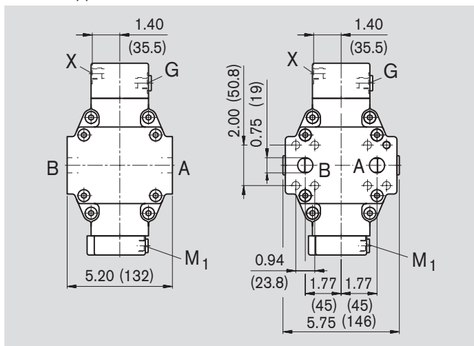
View Z
