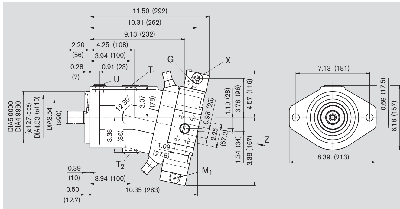
View Z
