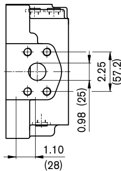
Detail V
