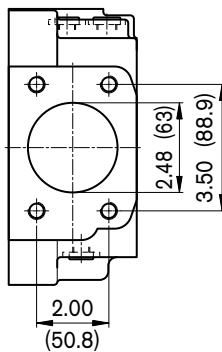
Detail W
